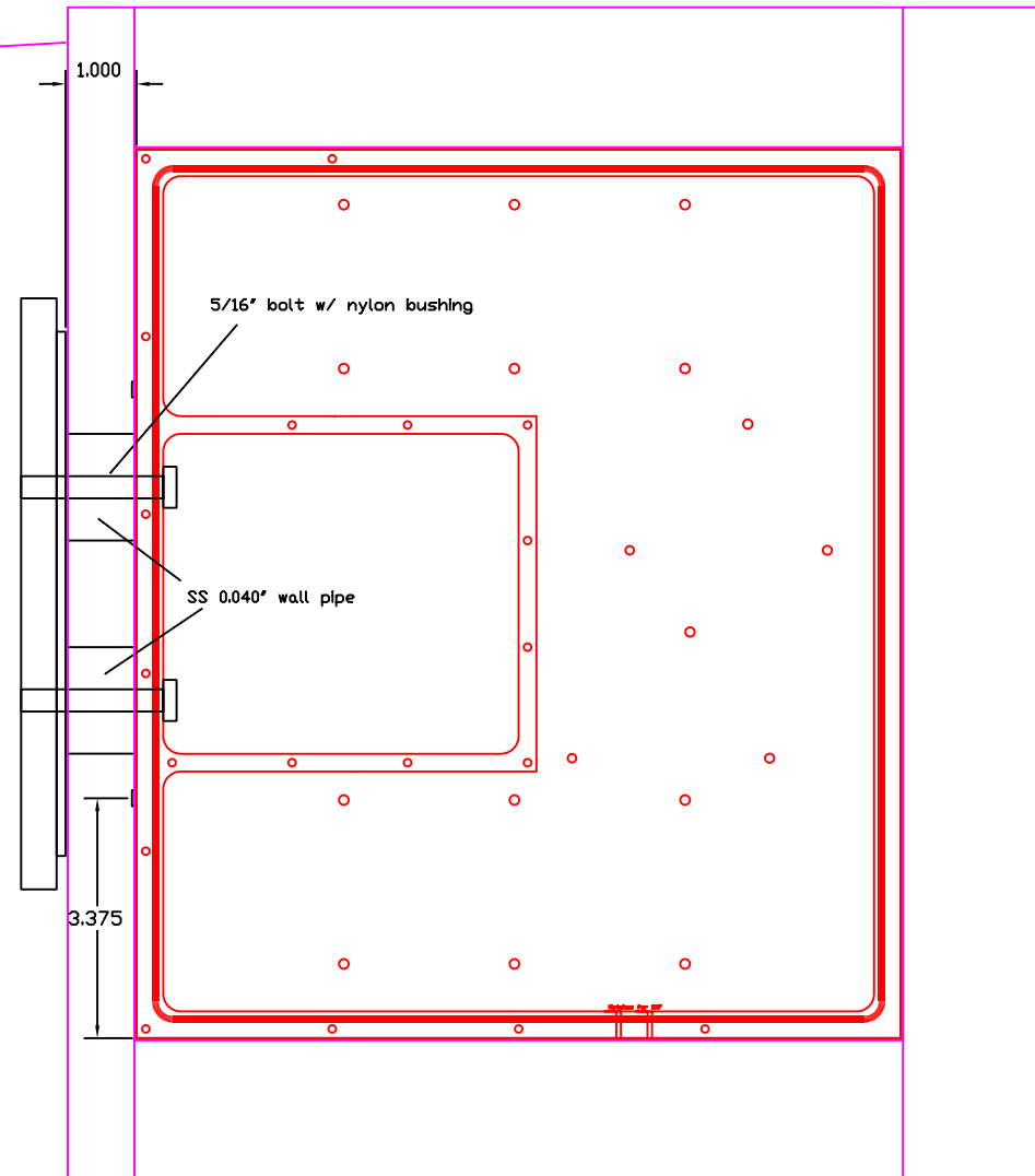
Top View
